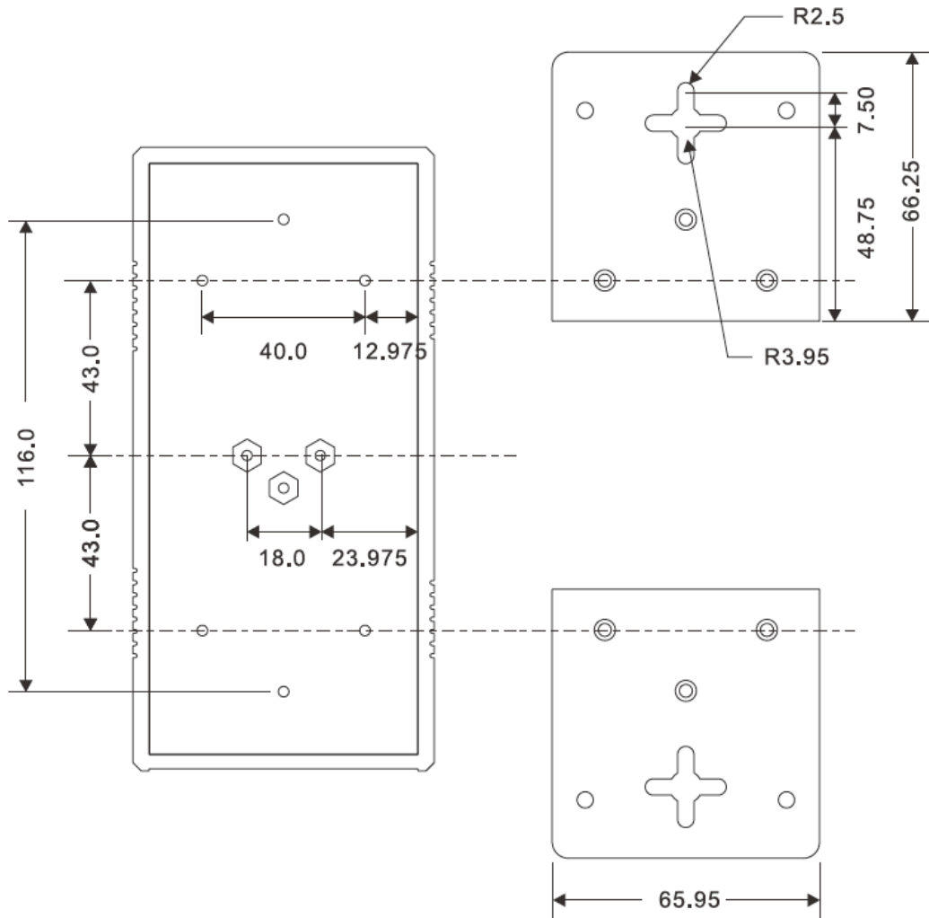
Wall-Mounting size
